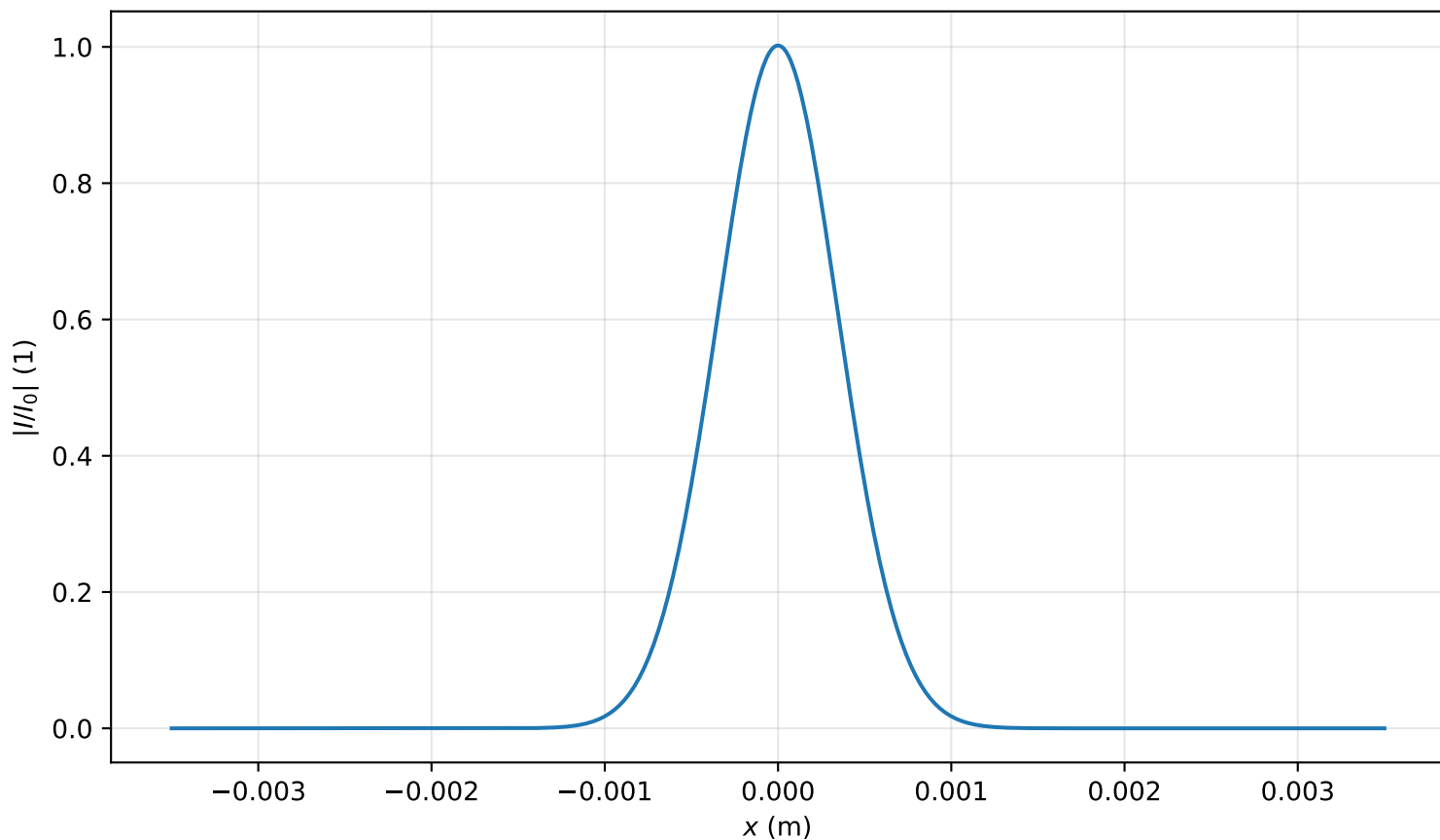
Intensity profile I(x, y = 0, z = 0.239m)/I_0 , P_{in}=0.3P_{cr} , artificial time
